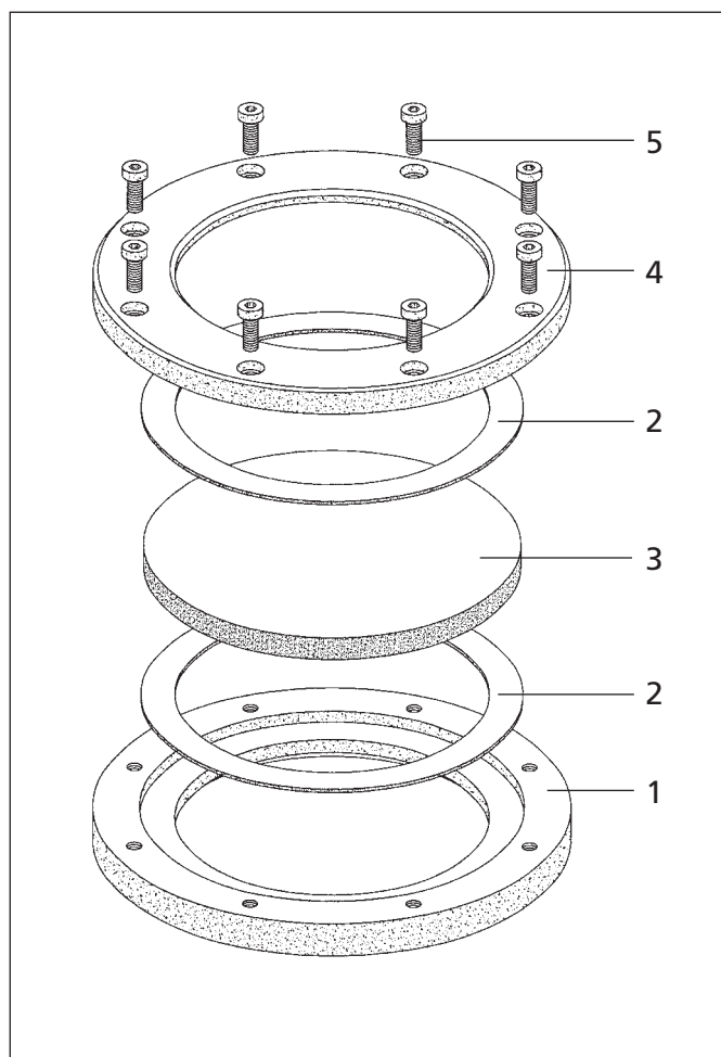
Exploded view of circular sight glass fitting in stainless steel
